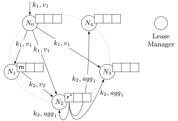
Figure 2: Execution of an initial insert and one \text{map}/\text{reduce}^* step (Replication shown)
